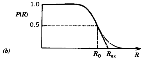
FIGURE 20.3 (a) Distribution of ranges for charged particles. (b) Probability of a particle having a range larger than R .
