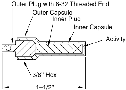
TYPE 193 GAMMA SOURCE CAPSULE ALL FUSION WELDED STAINLESS STEEL CONSTRUCTION
