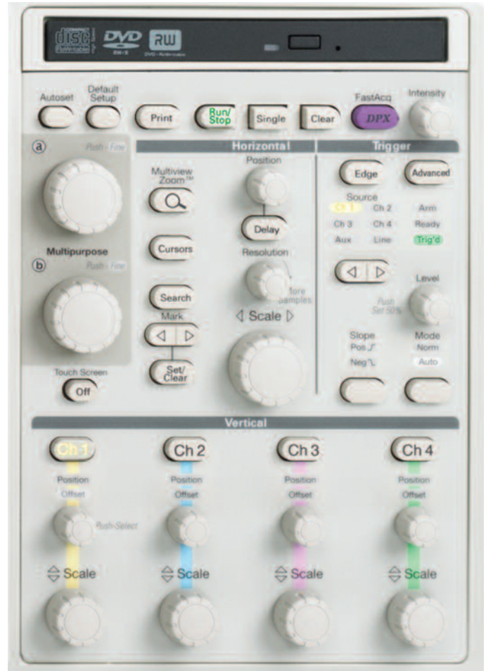
Figure 22. Front-panel control section of an oscilloscope.
