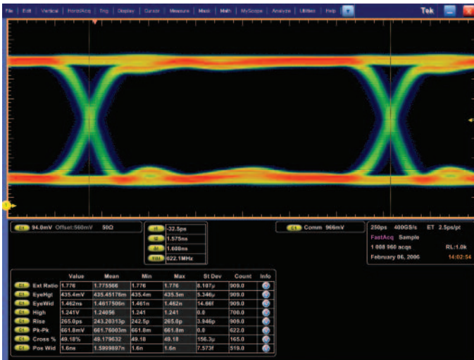
Figure 10a. 622 Mb/s serial data eye pattern.
