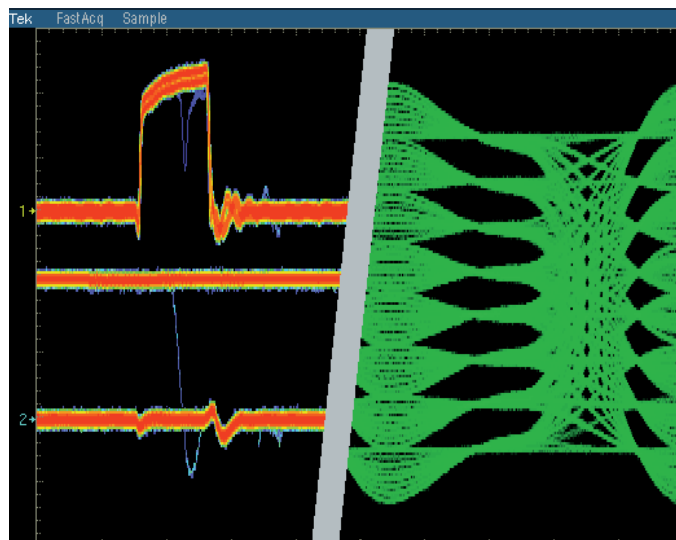
Figure 19. Some DPOs can acquire millions of waveform in just seconds, significantly increasing the probability of capturing intermittent and elusive events and revealing dynamic signal behavior. Left half is representative of a DPO display and the right half represents a typical DSO display.
