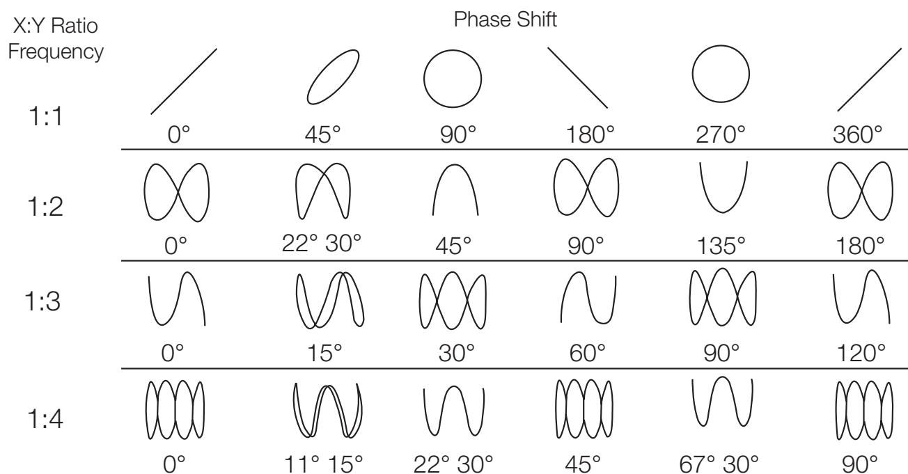
Figure 70. Lissajous patterns.
