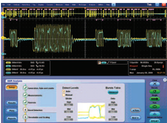
Figure 57. Advanced DDR Analysis tool automates complex memory tasks like separating read/write bursts and performing JEDEC measurements.
