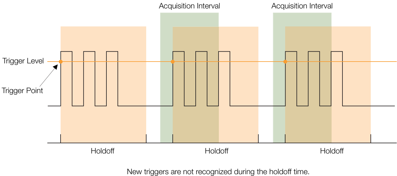
Figure 37. Trigger holdoff.
